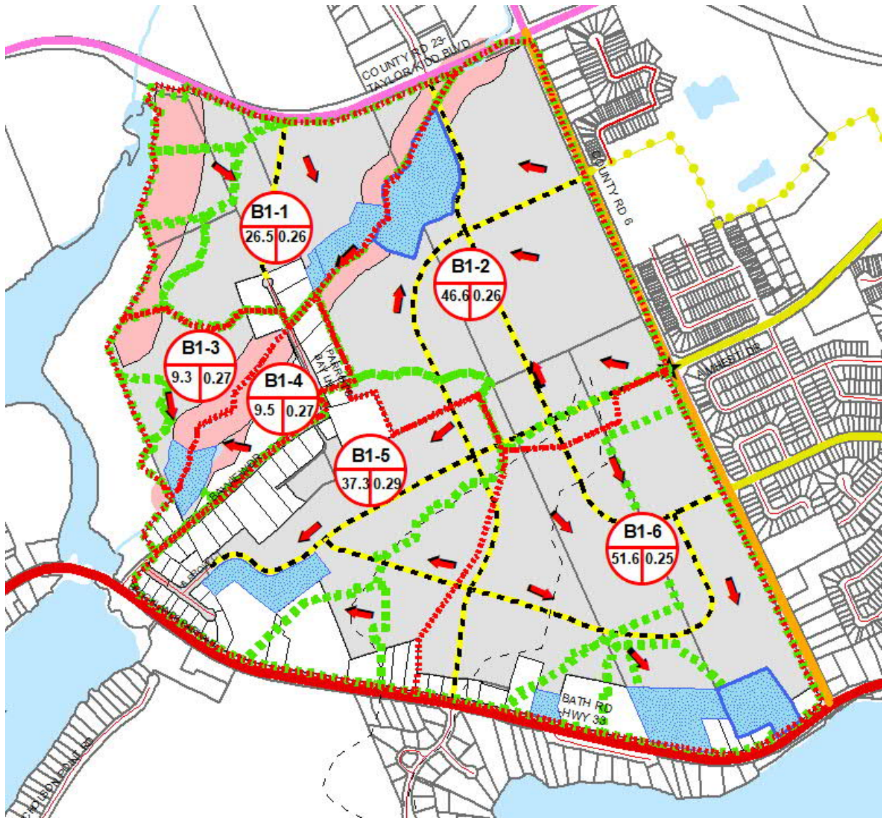
Figure 4 – Amherstview West Secondary Plan Post-Development Sub-Catchments Areas – Existing Conditions
