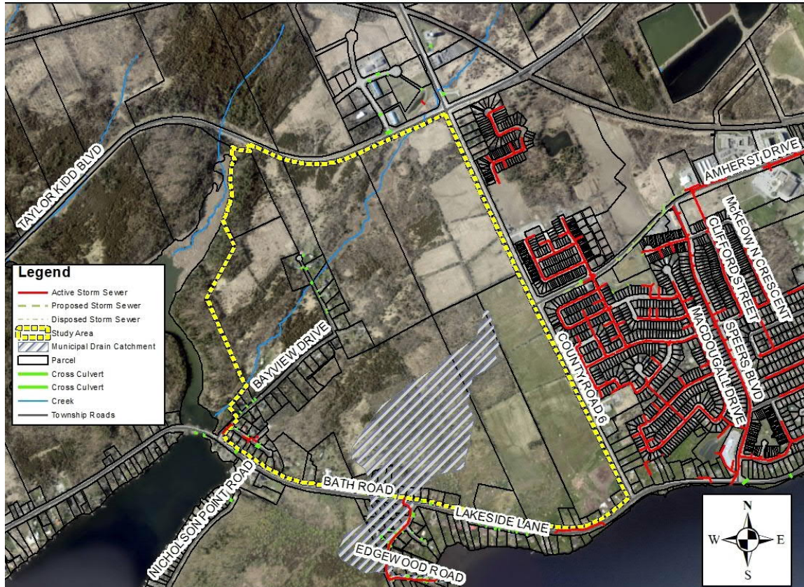
Figure 2-2: Edgewood Municipal Drain Catchment Area
